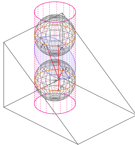
図 3.13: http://www.texample.net/tikz/examples/dandelin-spheres/
