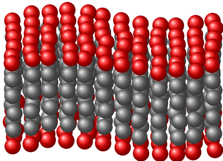
図 3.12: http://www.texample.net/tikz/examples/membrane-surface/
