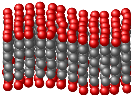
図 3.12: http://www.texample.net/tikz/examples/membrane-surface/
