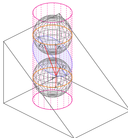
図 3.13: http://www.texample.net/tikz/examples/dandelin-spheres/
