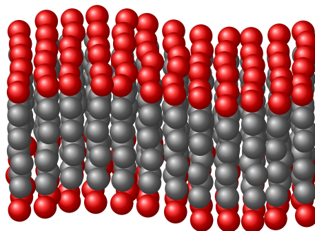
図 6.12: http://www.texample.net/tikz/examples/membrane-surface/
