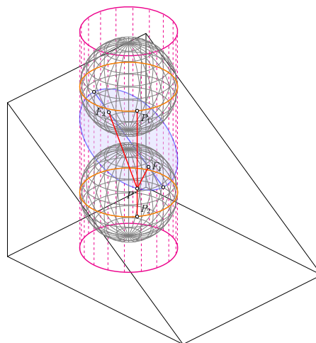
図 6.13: http://www.texample.net/tikz/examples/dandelin-spheres/
